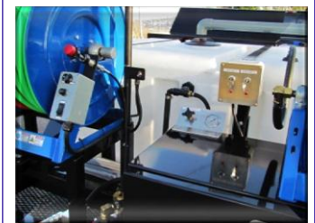
All Operational controls are mounted near the Jetting Reel for easy operation
